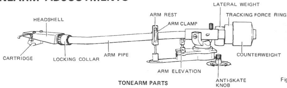
TONEARM PARTS
